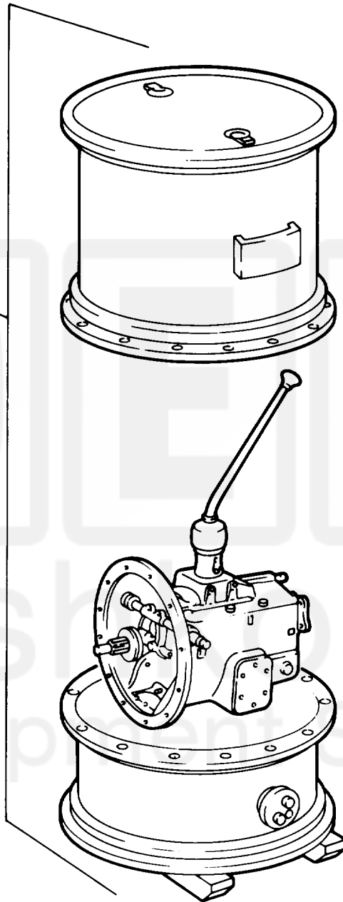
Figure 134. Transmission and Container Assembly.
